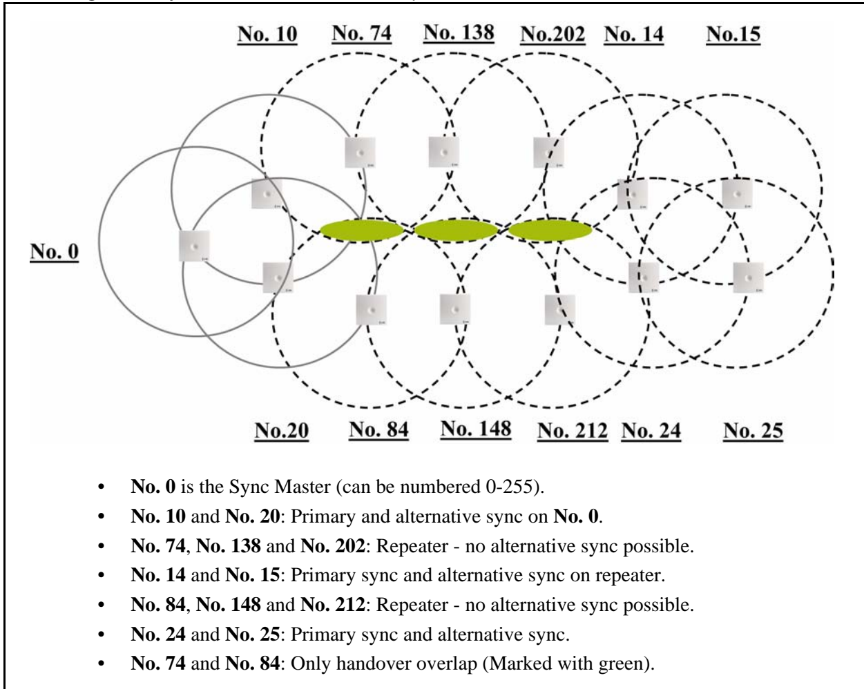
Figure 9 Synchronization Chain With Repeaters
